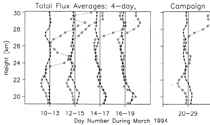
Figure 8. Same as Figure 7, but for the March 1994 campaign.
