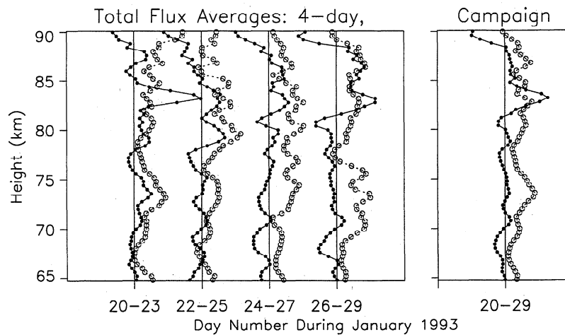
Figure 15. Overlapping 4-day and campaign estimates of zonal momentum flux (open dots) and meridional momentum flux (solid dots) in the mesosphere for the January 1993 campaign. Profiles are offset by 10 \text{ m}^2 \text{ s}^{-2} .
