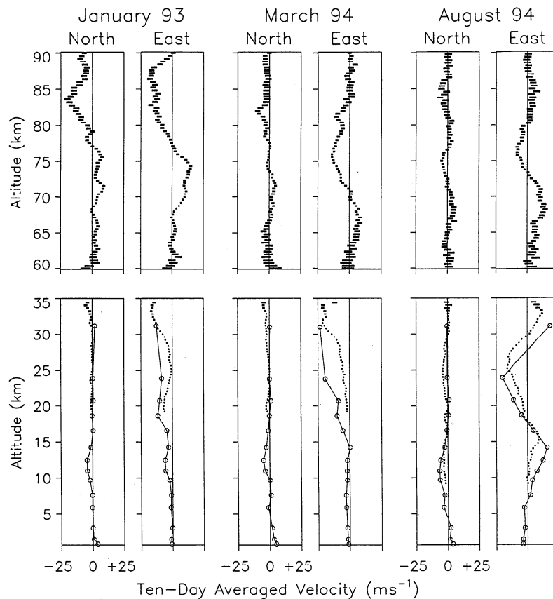
Figure 1. Campaign averages of the radar winds in the stratosphere and mesosphere during the three Jicamarca experiments (error bars as symbols) and averages of ECMWF winds for the coordinates of Jicamarca (open dots).
