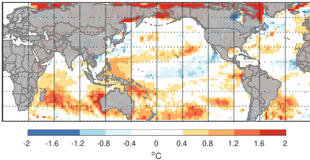
SST anomaly for APR 2025
