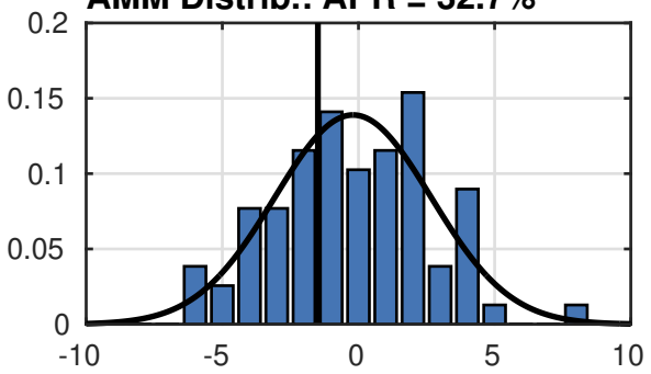
AMM Distrib.: APR = 32.7%
