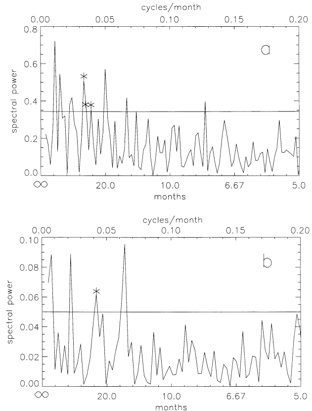
FIG. 4. (a) Spectral power of monthly mean anomalous OLR between 5^{\circ}\text{N} and 5^{\circ}\text{S} . Only OLR emitted by deep convection (raw values <240 \text{ W m}^{-2} ) in the chronically convective regions was included in the zonal means. (b) Spectral power of monthly mean anomalous HRC between 5^{\circ}\text{N} and 5^{\circ}\text{S} . Horizontal lines represent 95% confidence levels (the mean power for all periods plus two standard deviations). The asterisks indicate significant power at QBO periods. Power for periods less than 5 months is not shown.
