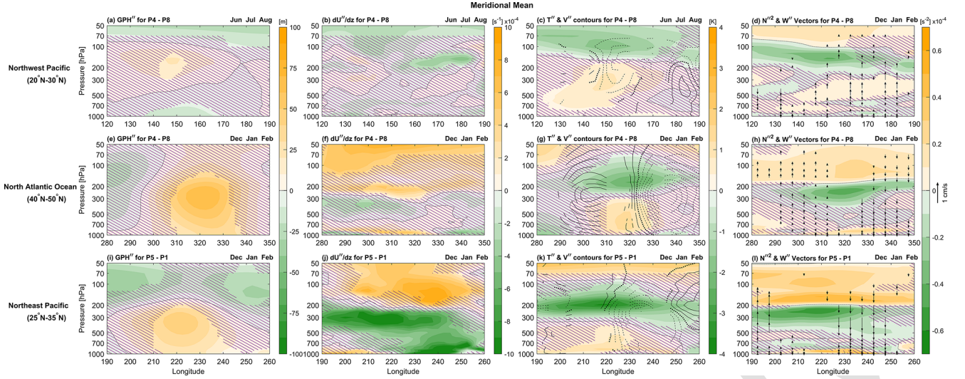
Figure 10. Longitude-pressure sections of composite differences between opposite QBO phases for selected latitudinal means shown in Figs. 7, 8, and 9. The top row shows the latitudinal mean between 20 and 30° N over the Northwest Pacific (120–190° E) during JJA, the middle row shows the mean between 40 and 50° N over the North Atlantic Ocean (280–350° E) during DJF, and bottom row shows the mean between 25 and 35° N over Northeast Pacific (190 and 260° E) during DJF. The first, second, third, and fourth column of each row represent the composite difference of GPH'', vertical shear of zonal wind ( dU/dz ), T'' (color bar) with V'' wind (contour lines at 0.5 m s -1 ), and N''^2 with W'' wind vectors, respectively. The top two rows use QBO W – E at 50 hPa (P4 – P8), and the third uses 70 hPa indices (P5 – P1). Violet cross-hatching indicates regions of statistical significance less than 90 %. The V'' contours on the 3rd column and W'' wind arrows on the 4th column are plotted only if either component's statistical significance exceeds the 90 %.
