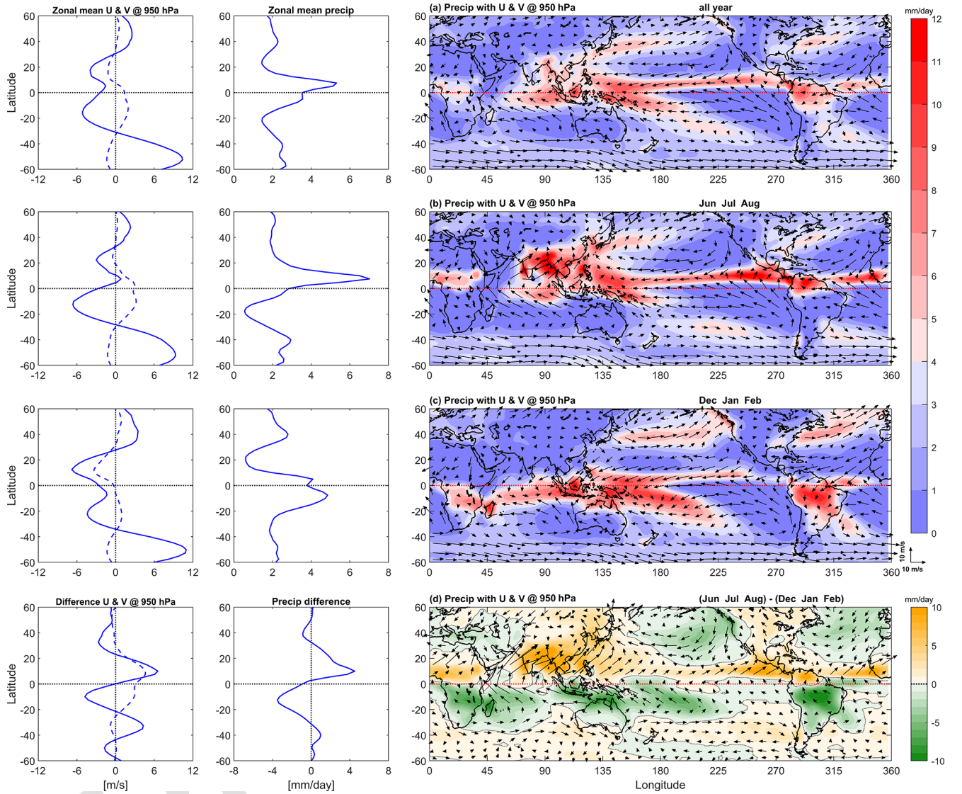
Figure 2. ERA-5 climatology (1979–2020) of precipitation ( P ) and horizontal winds ( U , V ) at 950 hPa, using only neutral ENSO months. The 1st and 2nd columns show latitudinal profiles of zonal mean zonal [ U ] (solid line) and meridional [ V ] (dashed line) winds, and zonal mean precipitation [ P ], respectively. The 3rd column shows charts of precipitation P (color bar) along 950 hPa wind vectors. From top to bottom, rows show results for the climatological (a) annual mean, (b) boreal summer monsoon (JJA), (c) austral summer monsoon (DJF), and (d) the composite difference JJA – DJF, respectively. In panel (d), a positive value (golden color) denotes enhanced precipitation during JJA relative to DJF, and a negative value (green color) denotes enhanced precipitation during DJF relative to JJA.
