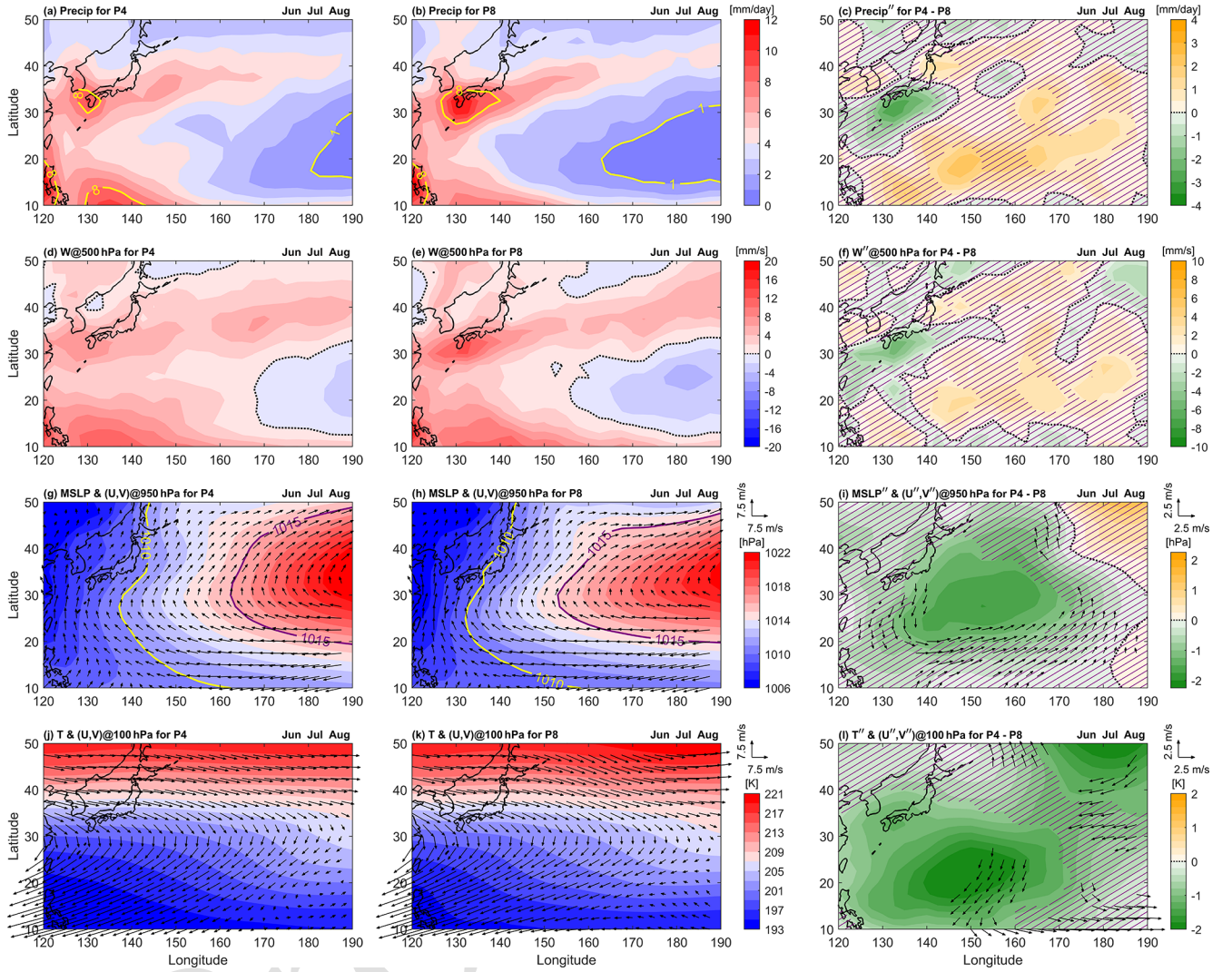
Figure 7. QBO regional teleconnection manifestation in the Northwest Pacific (10–50° N, 120–190° E) during boreal summer (JJA), showing composite climatologies of (left) QBO W at 50 hPa (P4), (middle) QBO E at 50 hPa (P8), and (right) QBO W – E at 50 hPa (P4 – P8), for (a–c) precipitation, (d–f) mid tropospheric W-wind at 500 hPa, (g–i) MSLP with ( U , V ) wind at 950 hPa, and (j–l) 100 hPa temperature with ( U , V ) wind. The violet cross hatching on the composite difference plots indicates regions of statistical significance less than 90 %. Wind anomalies ( U'' , V'' ) are plotted only if either component's statistical significance exceeds 90 %.
